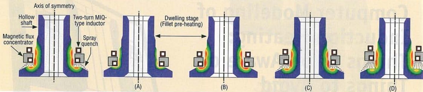
Fig. 2. Computer simulation of the sequential dynamics of induction scan hardening a hollow shaft using a two-turn machined integral quench (MIQ) inductor with an L-shaped magnetic flux concentrator ring (frequency = 9 kHz) (Courtesy of Inductoheat, Inc.)
