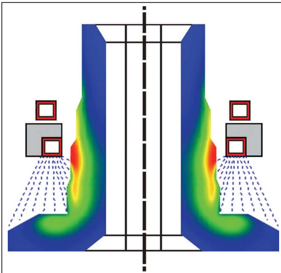
Fig. 3 — FEA computer modeling of vertical scan hardening of a hollow shaft. Courtesy of Inductoheat Inc.
