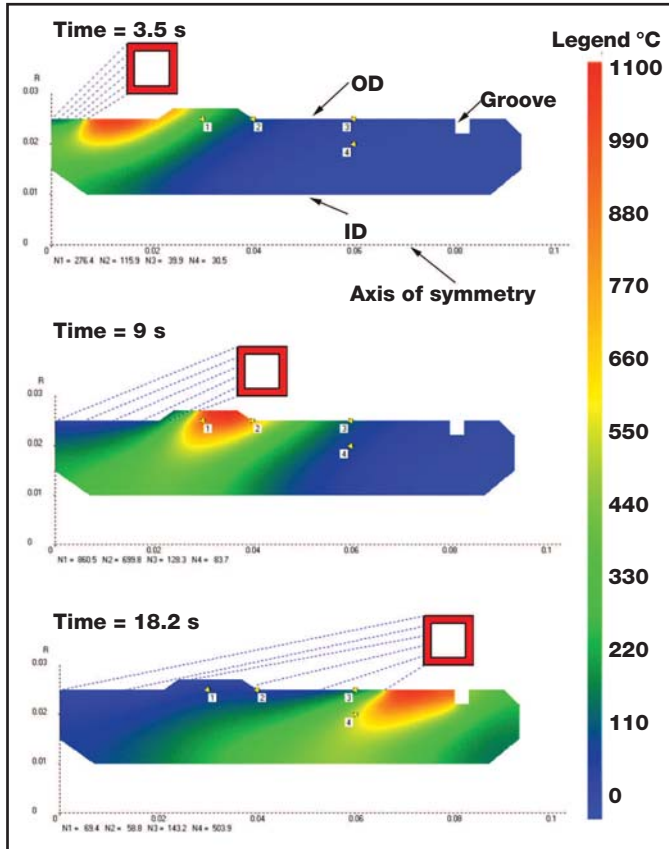
Fig. 4 — Computer modeling of sequential dynamics of induction scan hardening of hollow shaft with diameter changes, undercut, and groove. Courtesy of Inductoheat Inc.
