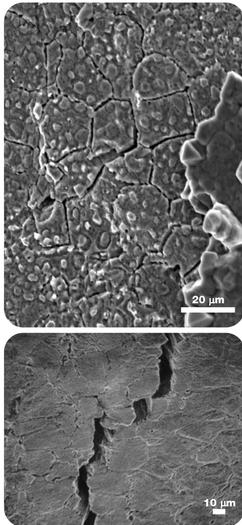
Fig. 1 — Grain boundary liquation (top) and cracking (bottom).
