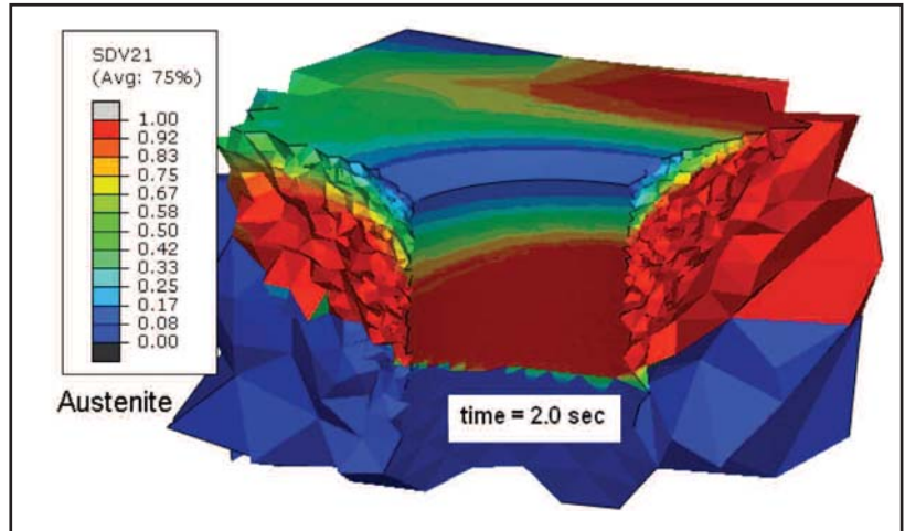
Fig. 6 — Computer prediction of austenite transformation. Courtesy of Deformation Control Technology Inc.
