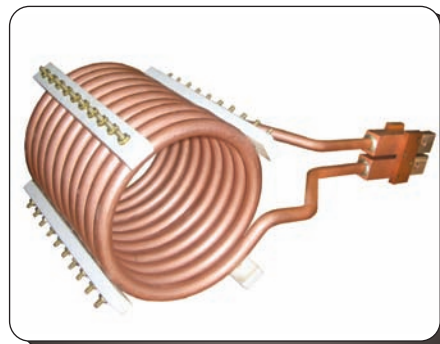
Fabricated multi-turn Inductors
