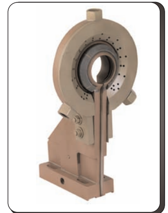
Machine Internal Quench Inductor
