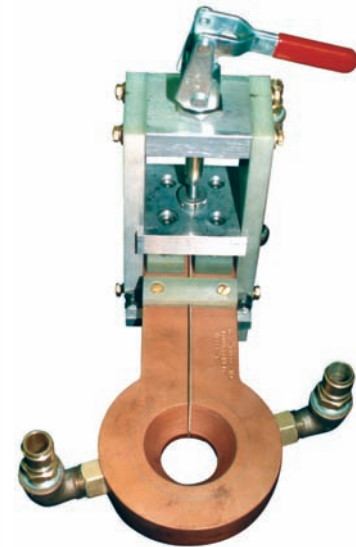
Insta-Change type coil and adapter
